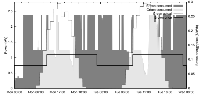
Figure 6. EAHadoop for FaceD workload and High-High days.
