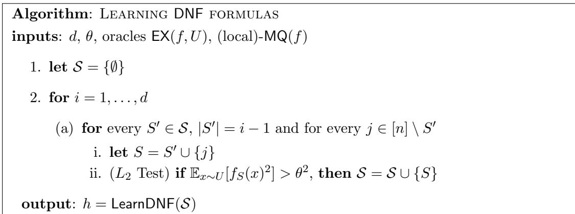
Figure 2: Algorithm: Learning DNF formulas under the Uniform Distribution
