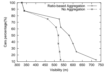
Fig. 9. Vehicle visibility
