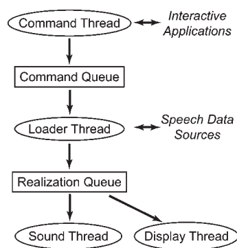
Figure 2. The architecture of RUTH.
