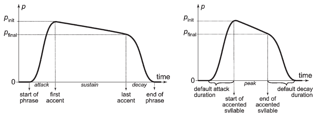
Figure 5. Action synchrony with speech. Underliner actions that synchronize with whole phrases (a, at left). Baton actions that synchronize with stressed syllables (b, at right).
