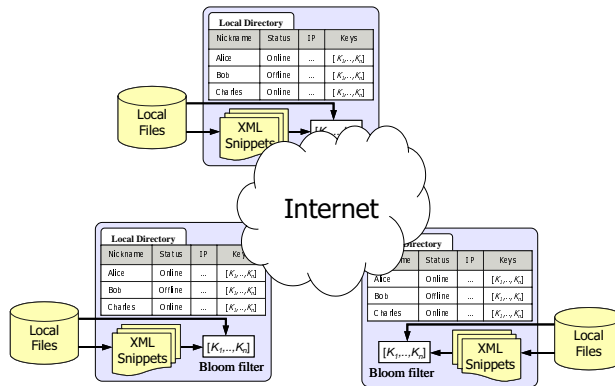
Figure 1. A PlanetP community is comprised of a dynamic set of peers connected by a network such as the Internet. Each peer has a local store of XML documents that it wishes to share with the community. Peers use a gossiping algorithm to help each other maintain a directory of currently active peers as well as a set of Bloom filters summarizing the content of peers' local stores.
