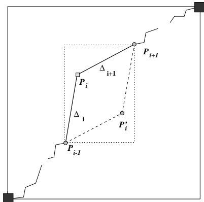
Figure 2: Permuting segments in monotone chains
