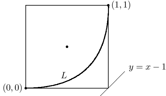
Figure 1: The limit shape L .
