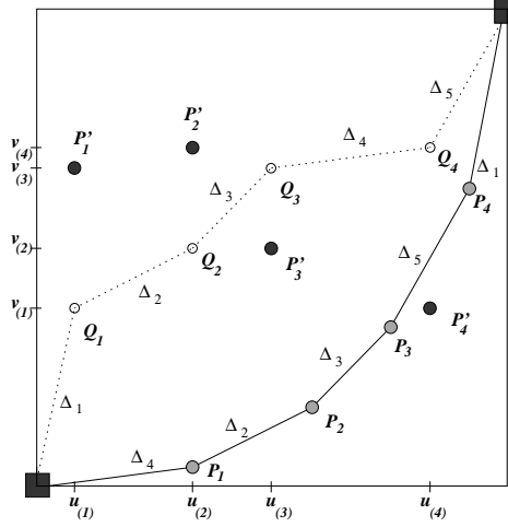
Figure 3: A sample of 4 points, its random monotone chain (dotted), and its convex chain (solid).
