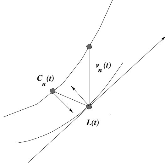
Figure 4: Area and Hausdorff distance.
