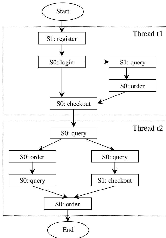
Figure 2: A Composed Service
