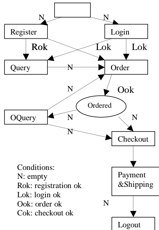
Figure 1: Behavior of A Seller Agent
