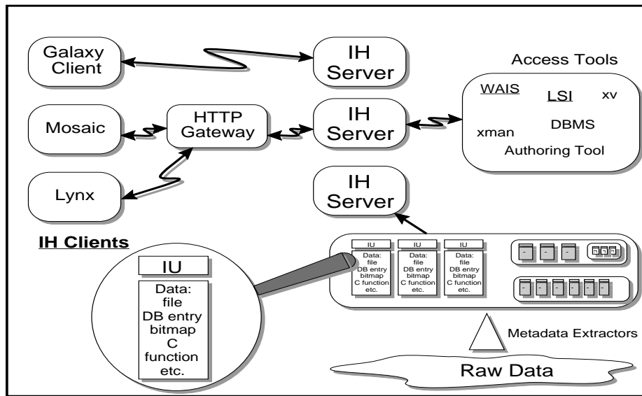
Fig. 3. InfoHarness Architecture.
