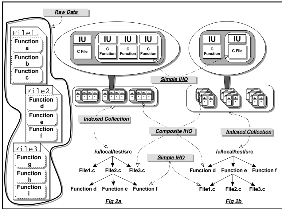
Fig. 2. Metadata Extraction for C code.
