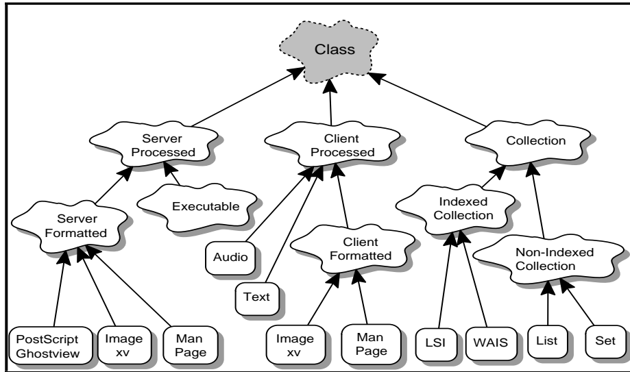
Fig. 1. InfoHarness Class Hierarchy with Sample Terminal Classes.
