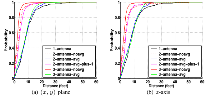
Fig. 6. Localization stability using ABP.
