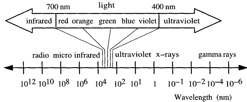
Figure 2.1: Electromagnetic spectrum.
