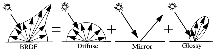
Figure 2.12: Reflectance components.
