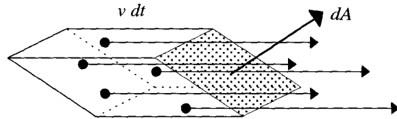
Figure 2.4: Total particles crossing a surface.
