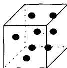
Figure 2.3: Particles in a differential volume.
