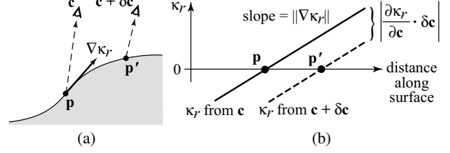
Figure 3: Suggestive contours and camera motion. (a) In a normal slice of the surface that contains \nabla \kappa_r (but not the camera), as the camera moves from c to c + \delta c , a point on the suggestive contour slides from p to p' . (b) The distance p travels along the surface in the direction of \nabla \kappa_r depends on two factors: \kappa_r is offset by \partial \kappa_r / \partial c \cdot \delta c due to the camera motion \delta c ; and the slope of these lines denotes the local gradient magnitude of \kappa_r . These factors are the numerator and denominator, respectively, of equation (1).
