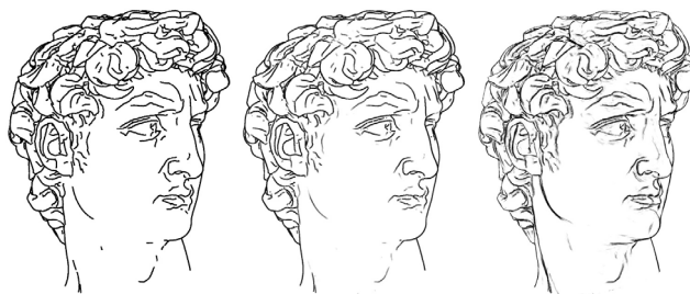
Figure 10: Different drawing styles produced by our interactive suggestive contour viewer. Left: constant-weight strokes. Center: faded strokes. Right: texture-mapped rendering. We find that the fading of strokes provided either explicitly (as at center) or implicitly due to interpolation within texture maps (as at right) helps the perceived frame-to-frame coherence.
