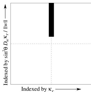
Figure 9: Texture map used to draw suggestive contours. We pass in \kappa_r and (\sin^2 \theta)D_w \kappa_r / \|\mathbf{w}\| as the texture coordinates at each vertex, so that the black texels are used for \kappa_r near zero and (\sin^2 \theta)D_w \kappa_r / \|\mathbf{w}\| > \epsilon .
