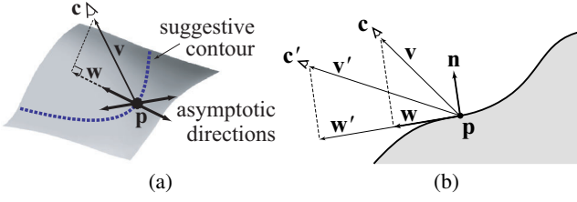
Figure 2: (a) w is the projection of the view direction v onto the tangent plane. At a suggestive contour, w points in one of the asymptotic directions of the surface—directions in which the curvature is zero. (b) Suggestive contours do not move when the camera motion is in the radial plane (from c to c' ) because the direction of w does not change (only the length of w' is different, not its direction)
