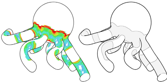
Figure 4: Comparison of density of suggestive contours considered over all viewpoints ( left ) with lines of zero Gaussian curvature, drawn in dark grey ( right ). Colors on left correspond to legend in Figure 1. Light grey shading on right indicates regions of negative Gaussian curvature. Note that suggestive contours can only occur in areas with K < 0 , but most frequently appear where K is near 0. White regions (never touched) correspond with areas where K > 0 .
