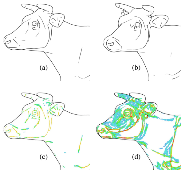
Figure 1: Suggestive contours in a dynamic scene: (a) contours and suggestive contours seen from view A; (b) seen from view B; (c) distribution of faces touched by suggestive contours as camera moves from A to B; and (d) distribution of faces touched for views uniformly distributed over the sphere.
