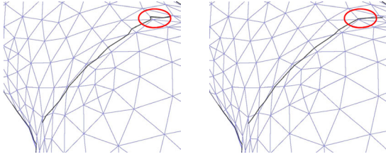
Figure 7: Low-resolution model with suggestive contours found using linear (left) or cubic Hermite (right) interpolation. The latter approach uses not only the value but also the gradient of \kappa_r at each vertex to improve the estimated locations of \kappa_r = 0 .
