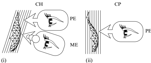
Figure 14. The shear in the case of observer AK, stimulus (a), tasks CH and CP. A view of the pictorial relief in case of (i) task CH, (ii) task CP. The viewing direction of the physical eye (PE) is horizontal in both cases. The shear is visualised via families of equal-distance planes. In this case the depth stretch is not noticeable. (Otherwise this would show up in the spacing.) The viewing direction of the 'mental eye' (ME) is suggested as orthogonal to the equal-depth planes. In this case the shear's slant is 18^\circ . Notice the difference in pose in the two cases. The poses are very similar if you reckon in terms of the equal-distance planes. The shear indeed simulated a change of perspective.
