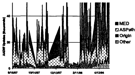
Fig. 4. Breakdown of BGP updates at the Mae-East exchange point.
