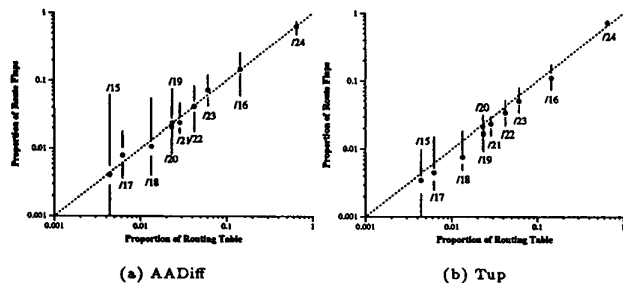
Fig. 7. This figure shows the proportion of routing updates versus prefix length for both AADiff and TUp events. The vertical axis represents the proportion of routing updates generated by a set of prefixes with identical length. For example, a /16 represents the proportion of updates generated by all prefixes of length 16. These data represent August 1996 at the Mae-East exchange.
