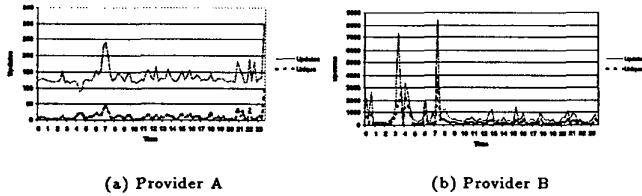
Fig. 8. Number of BGP updates and unique prefixes announced over the course July 10, 1998 at the Mae-East exchange point by two large service providers.
