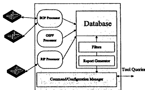
Fig. 1. Overview of the RouteTracker architecture.
