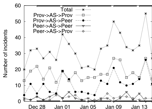
Figure 9: Probable export misconfiguration incidents per day.
