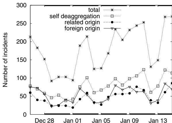
Figure 5: Probable origin misconfiguration incidents per day.
