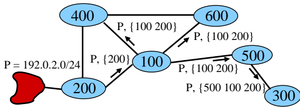
Figure 1: Border gateway protocol (BGP) network example.
