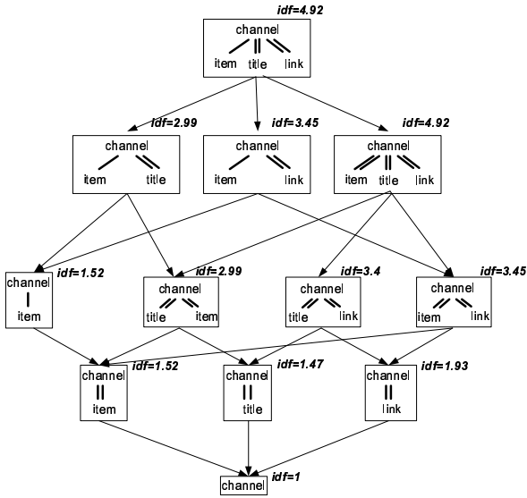
Figure 5: A Query Relaxations DAG for binary Scoring
