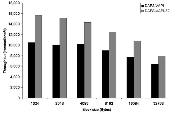
Fig. 7. Impact of Buffer/Descriptor Management
