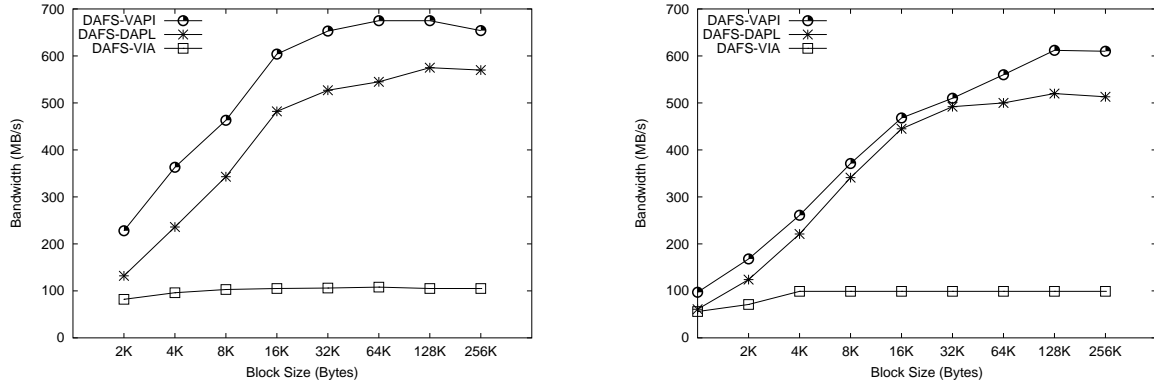
Fig. 4. Read (left) and Write (right) Bandwidth using Asynchronous I/O
