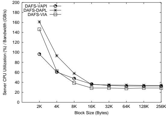
Fig. 5. Ratio of Server CPU Utilization to Read Bandwidth
