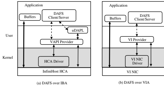
Fig. 3. DAFS Implementation Architecture
