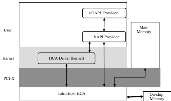
Fig. 2. Infiniband Architecture
