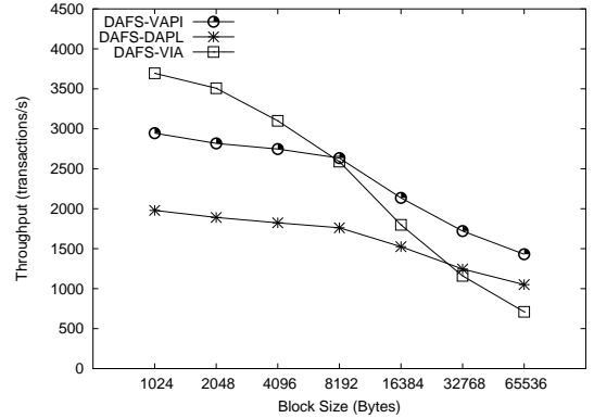
Fig. 6. Postmark Throughput
