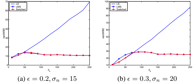
Fig. 7. The performance of the switching algorithm comparing to LS and LMS algorithms.
