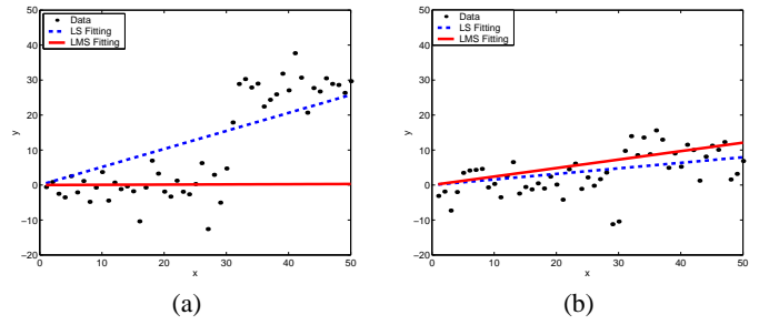
Fig. 6. Example linear regression demonstrating that LMS performs worse than LS when the inlier and outlier data are too close.
