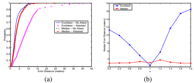
Fig. 8. (a) The CDF of the error distance for the NNSS method in Euclidean distance and in median distance, with and without an attack (one reading is modified to \alpha \cdot ss_i , where \alpha = 0.6 ). (b) Median of the error distance vs. the attacking strength \alpha (one reading is modified to \alpha \cdot ss_i ).
